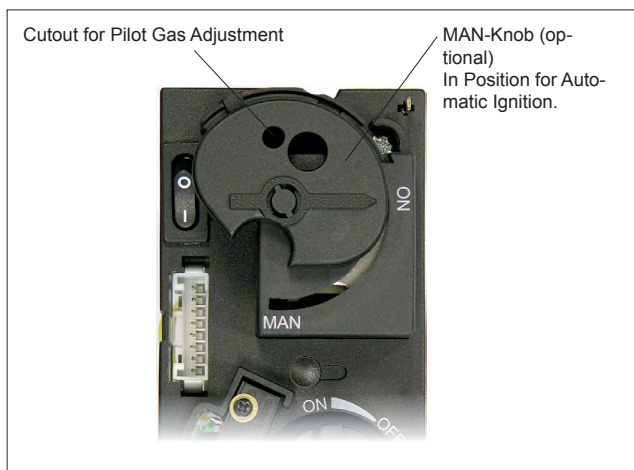
Figure 3: Combination Control, View MAN-Knob (optional)
